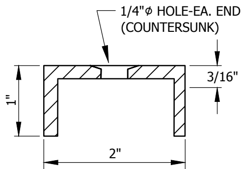
CHANNEL SECTION
