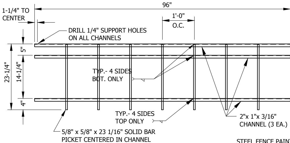
TYPICAL FENCE SECTION
