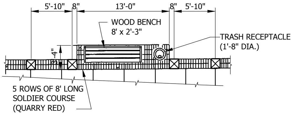
BENCH AREA DETAIL
