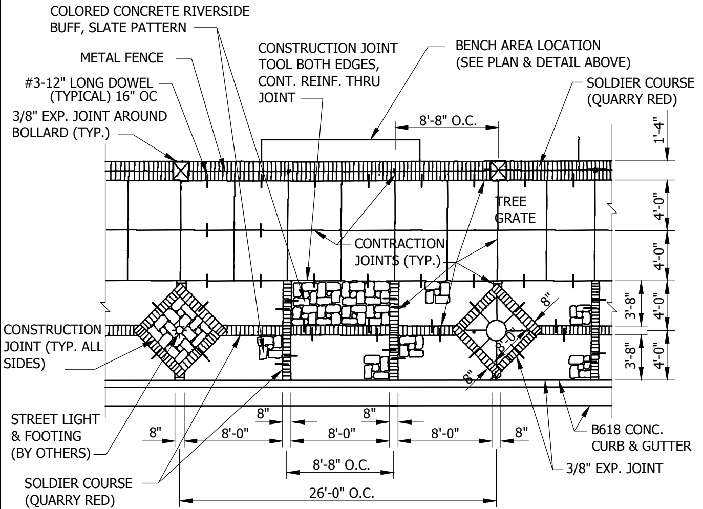
PLAN
