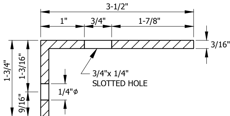
ANGLE BRACKET SECTION
